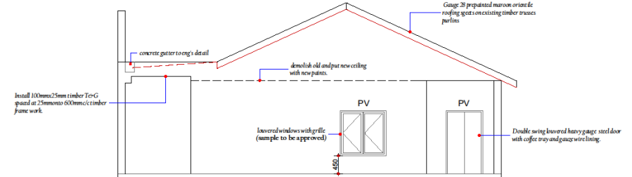
MASTER SIDE ELEVATION
