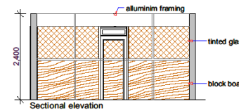
ALLUMINIUM PARTITIONING - POOL OFFICE
