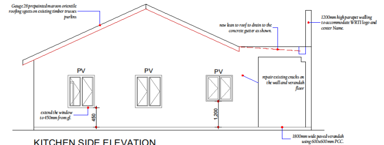
KITCHEN SIDE ELEVATION
